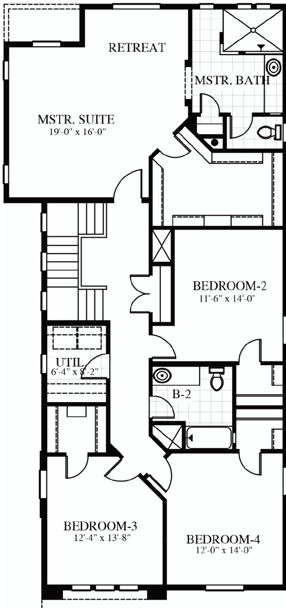
SECOND FLOOR
