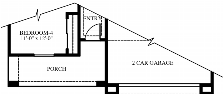
ELEVATION B FIRST FLOOR PLAN
