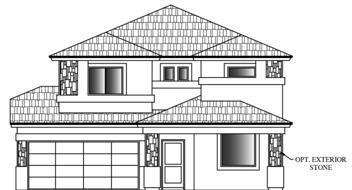
ELEVATION C
