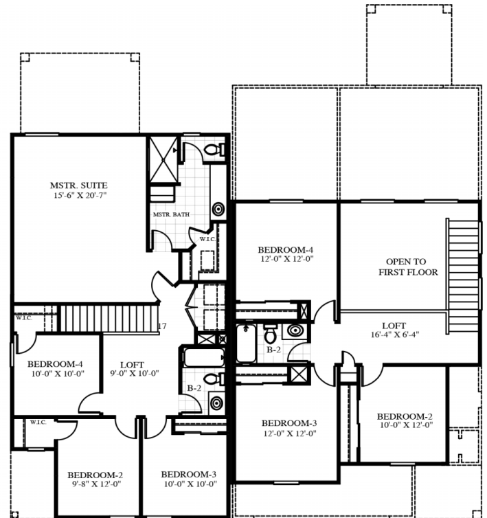
PLAN TH-3 SECOND FLOOR
