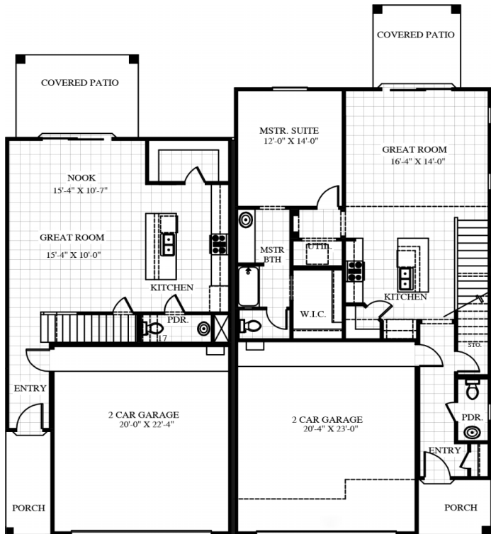
PLAN TH-4 FIRST FLOOR
