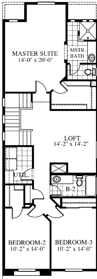
SECOND FLOOR
