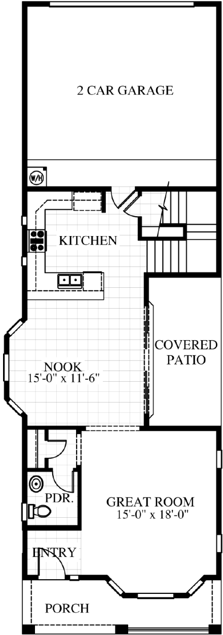
FIRST FLOOR
