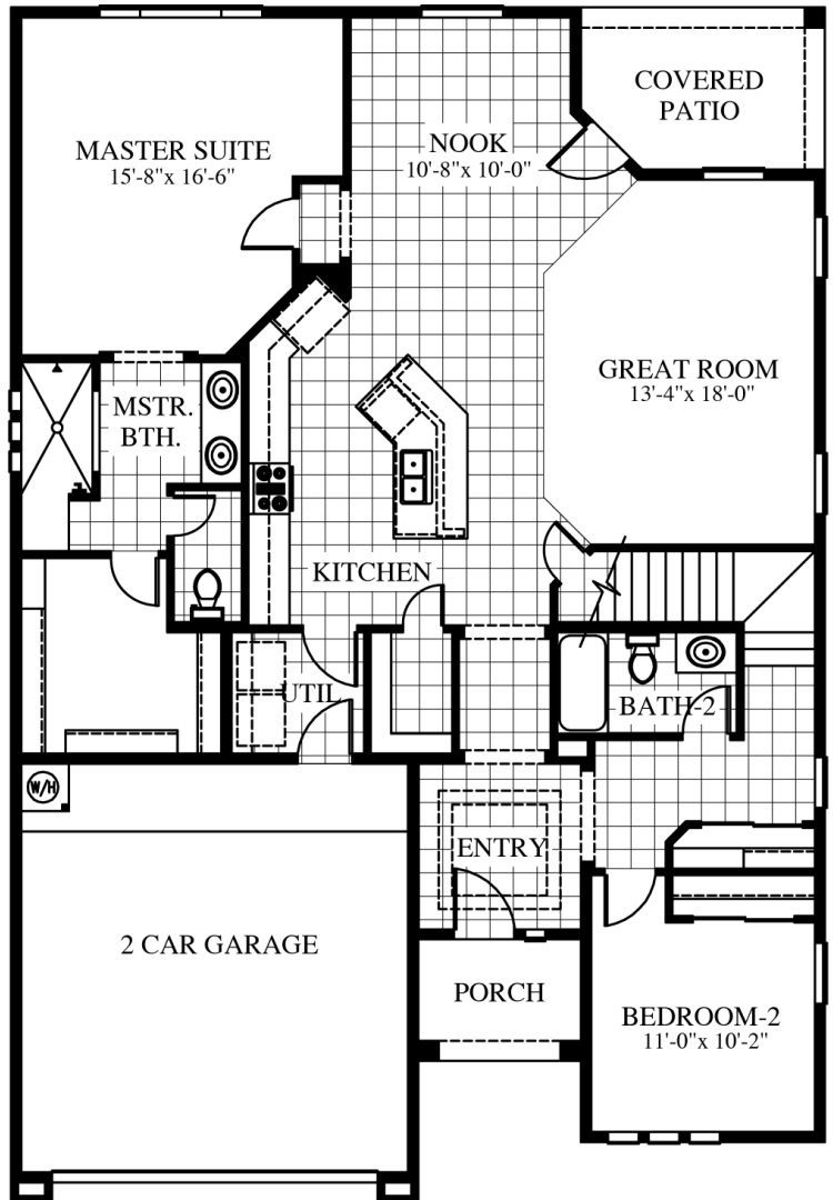
FIRST FLOOR
