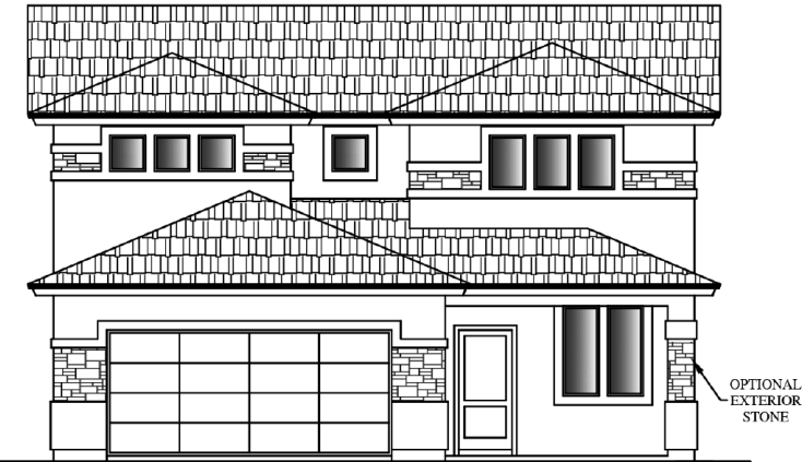
ELEVATION C
