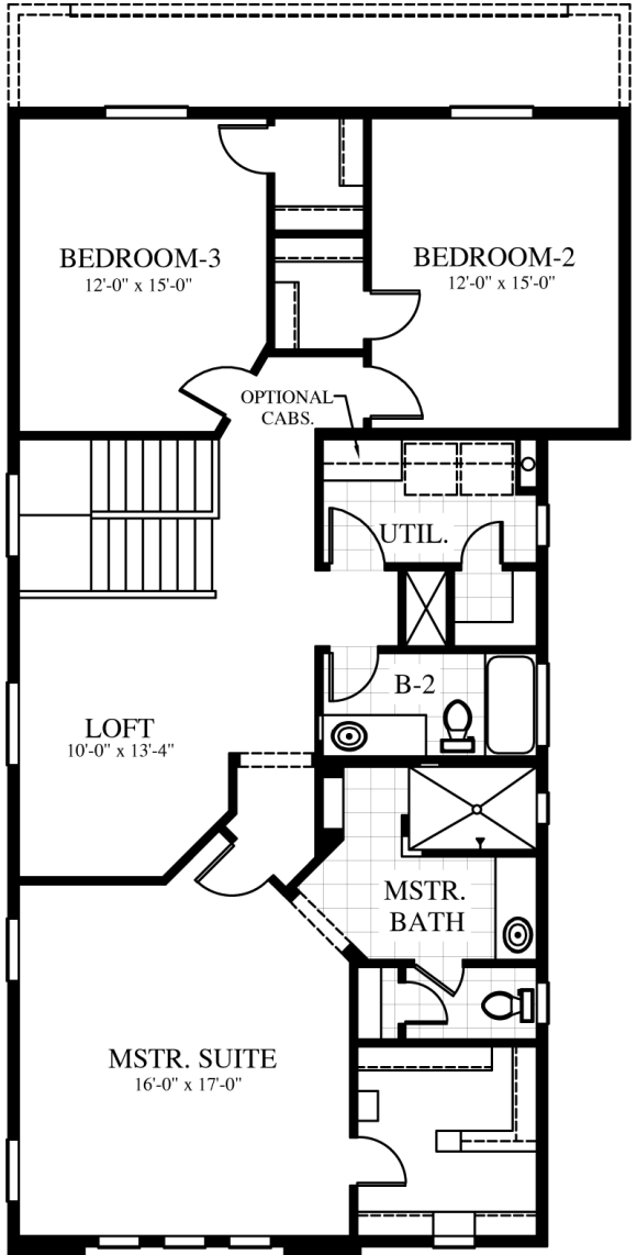
SECOND FLOOR
