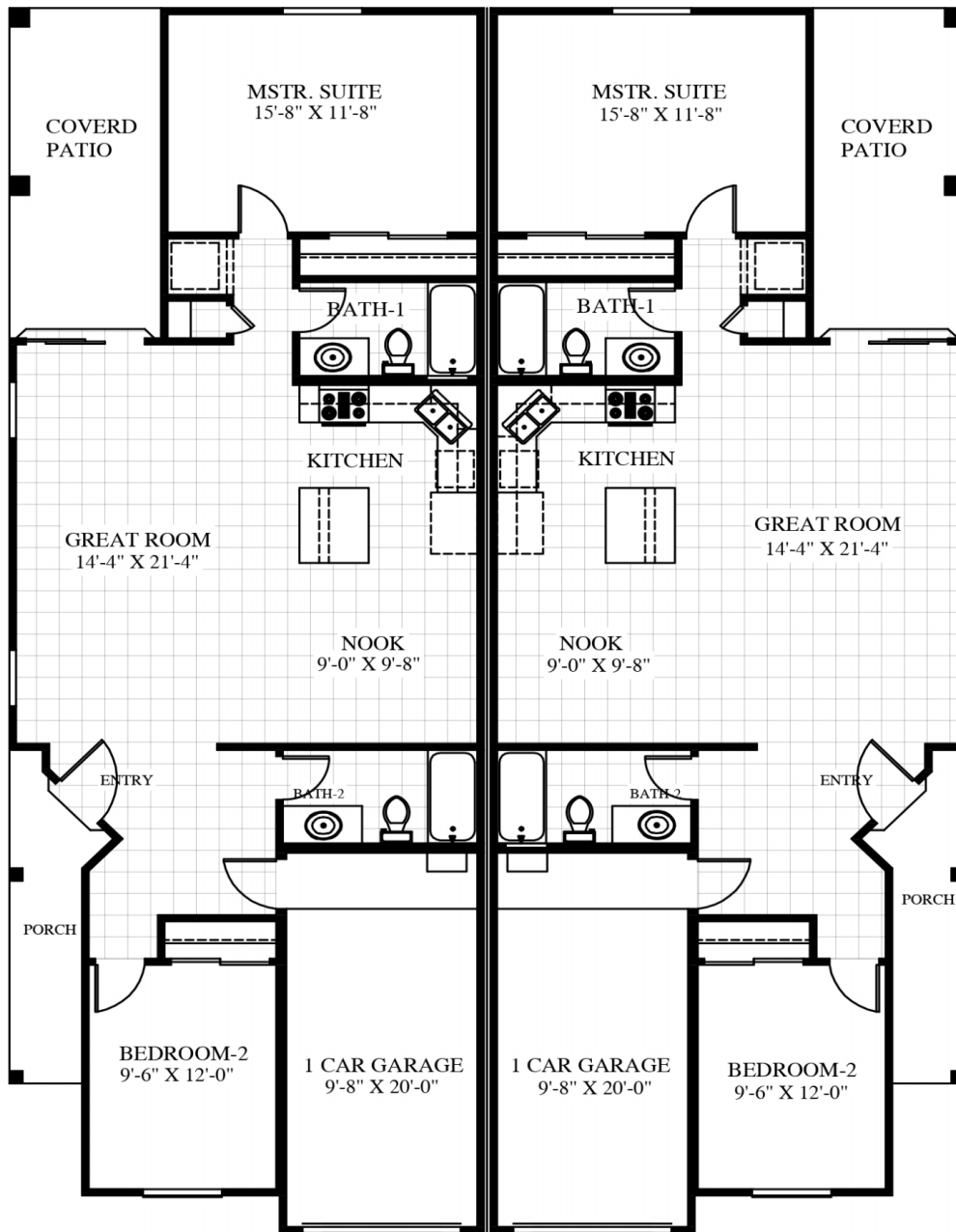
PLAN TH-1
