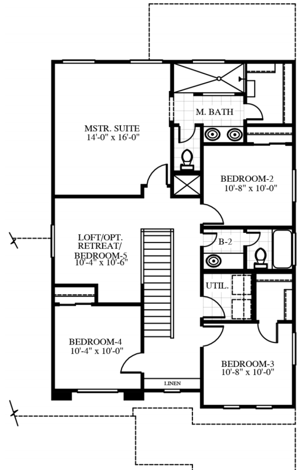
SECOND FLOOR
